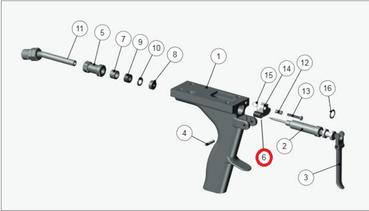
Figure 30: 7233-00 Handle Parts List
